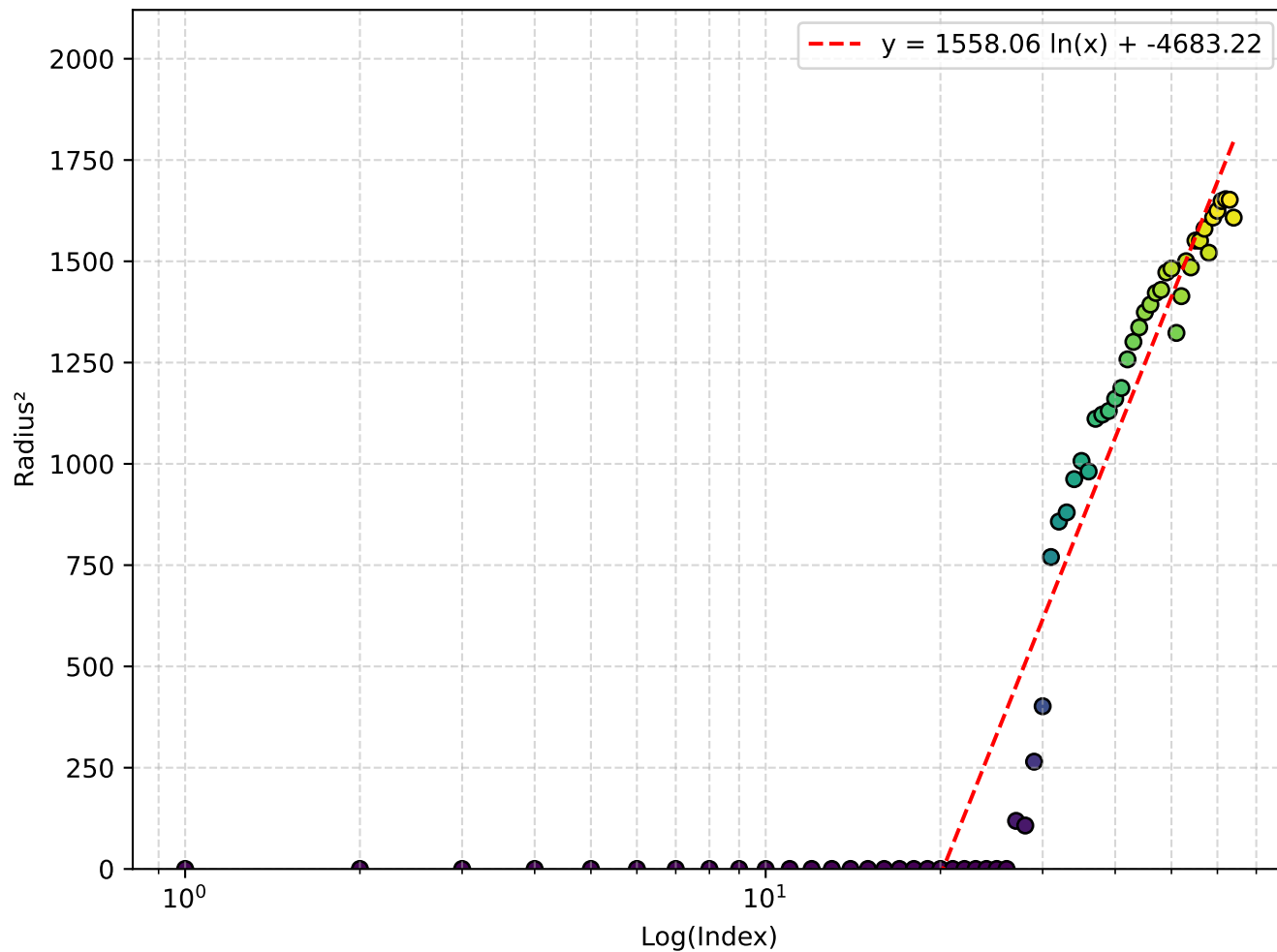
Liu Plot Run 019
